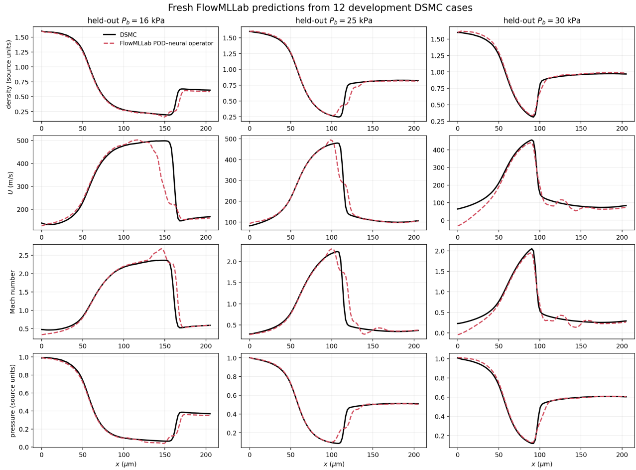
Figure 4: Centerline slices extracted from the new full-field FlowMLLab predictions for all three held-out back pressures. These curves are regenerated by qa/run_nozzle_field_validation.py .
