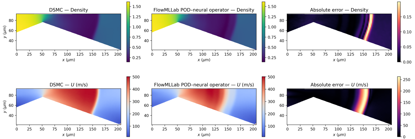
Held-out micro-nozzle case: P_b = 16 kPa (prediction generated by FlowMLLab)
