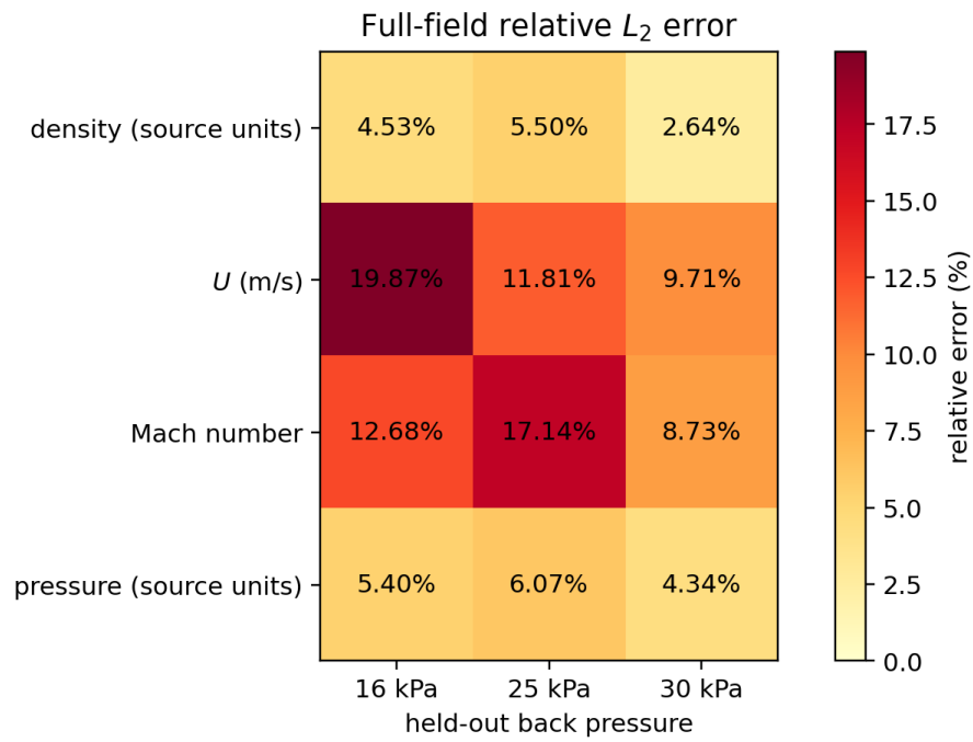
Figure 5: Full-field relative L_2 errors from the same fresh run. A single average would hide both the output dependence and the harder operating cases.
