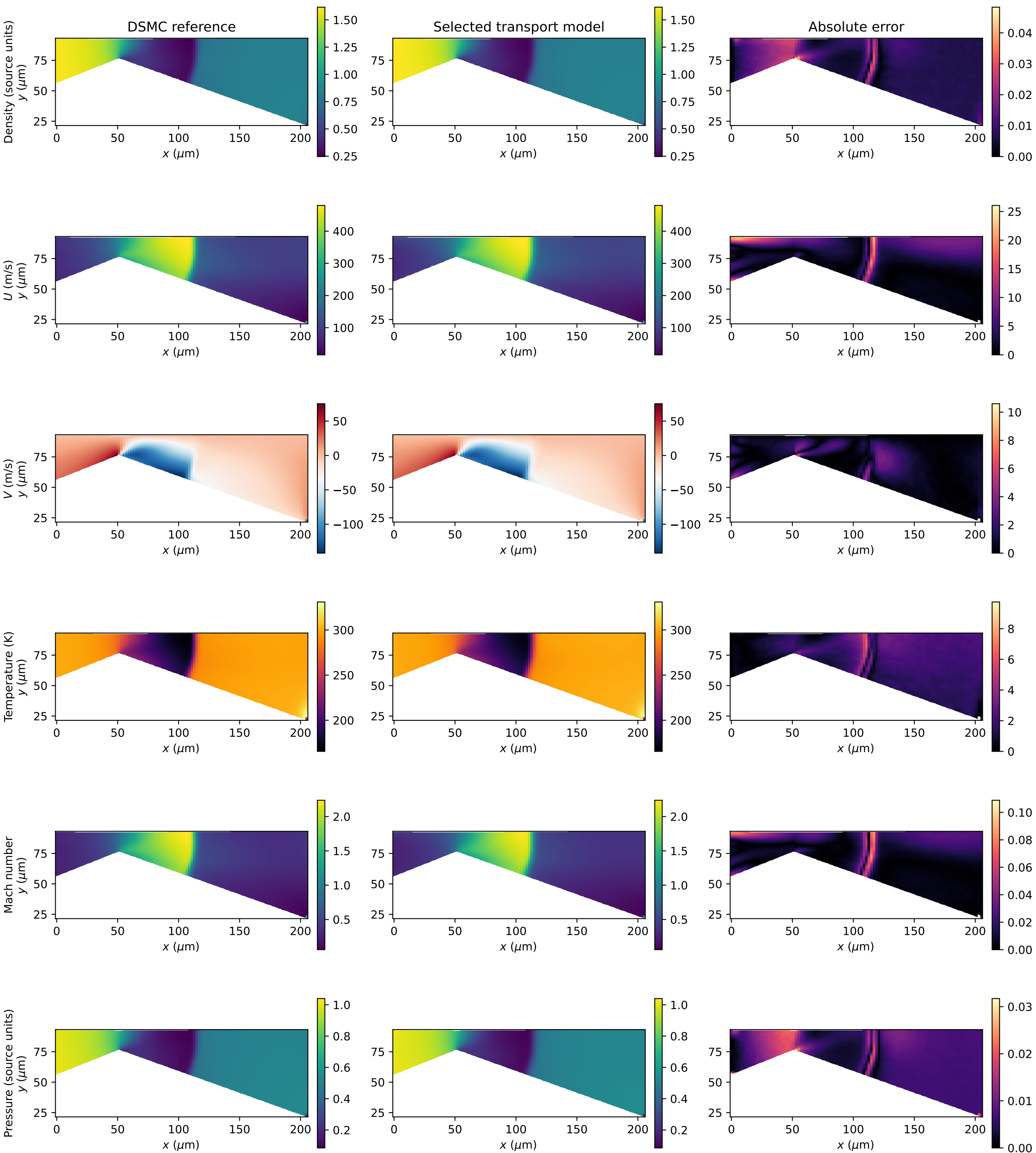
Micro-nozzle at 25 kPa | all six physical fields
