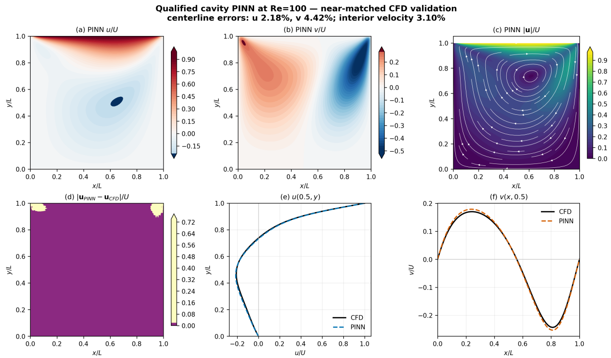
Figure 4. Qualified Re=100 PINN evidence regenerated from the accepted Unity checkpoint: velocity components, speed and streamlines, pointwise velocity error, and both CFD centerline comparisons. The large corner differences in panel (d) expose the regularized-versus-classical lid mismatch rather than being hidden by the domain-average metric.
