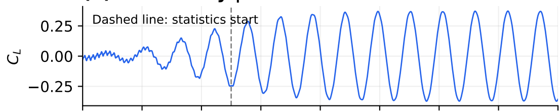
(b) Lift history | D40
