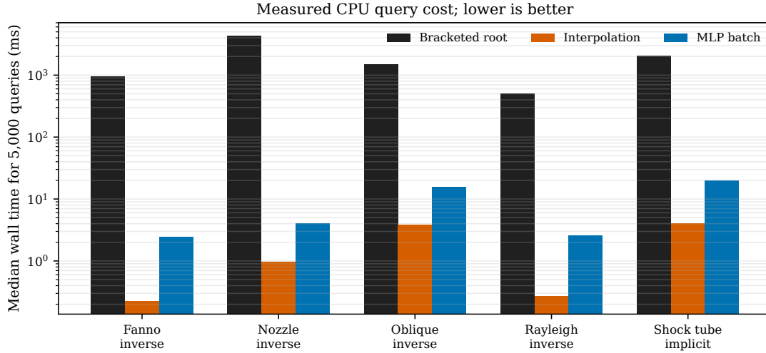
Figure 4: Measured CPU cost. Interpolation is fastest; batched MLP inference is substantially faster than repeated bracketed roots.
