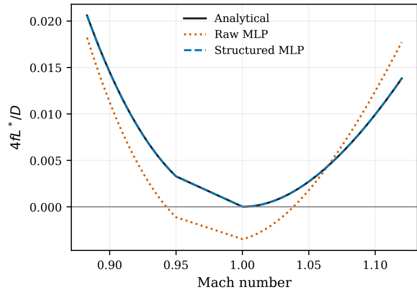
Near-sonic Fanno limit
