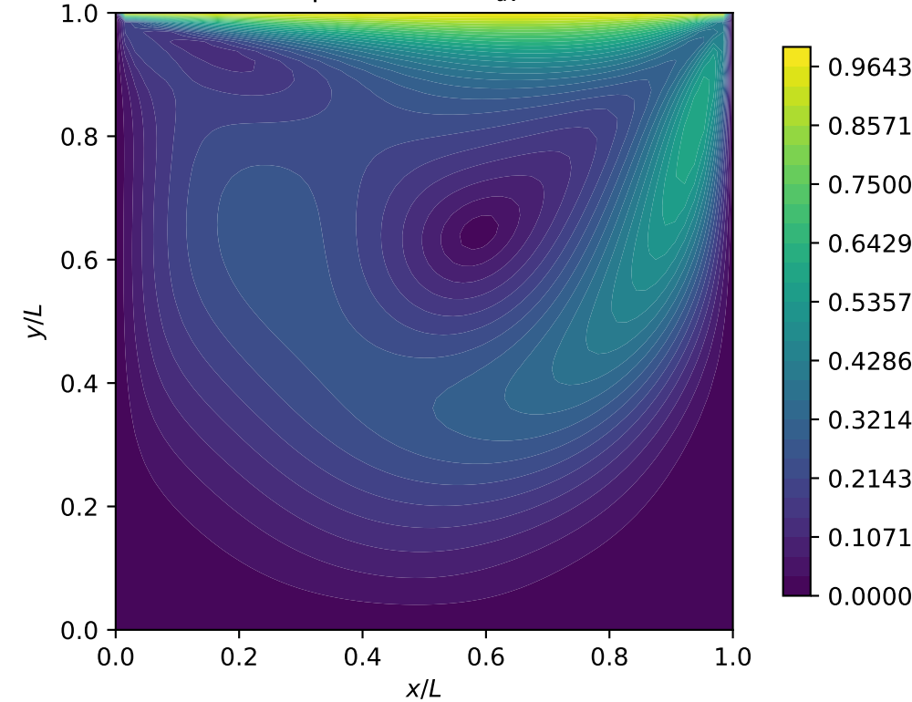
(e) Blind prediction; E_{uv} = 0.072\%
