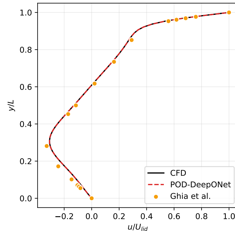
(e) Blind prediction; E_{uv} = 0.072\%
