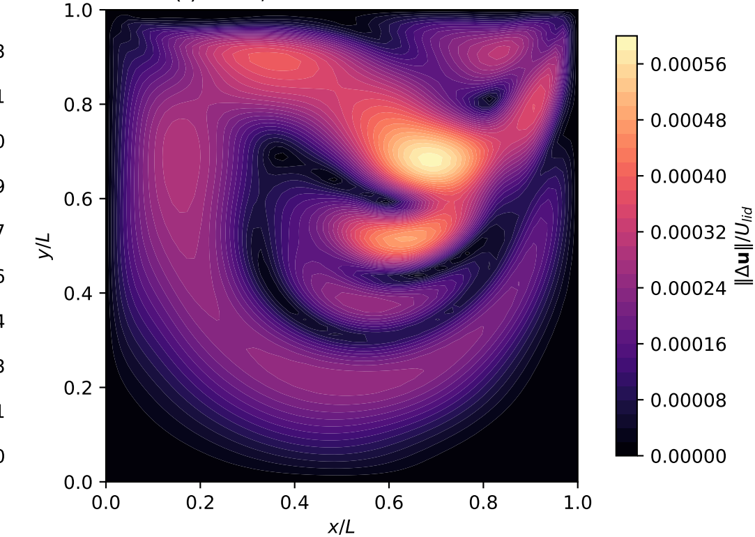
(f) Error; 0.80 ms vs CFD 8.5 s
