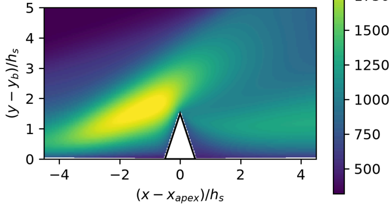
DSMC T
