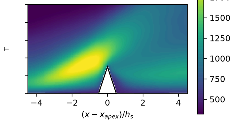
Predicted T
