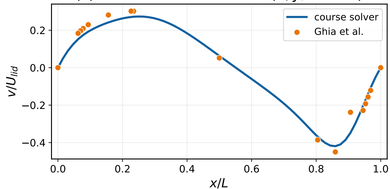
(c) Horizontal centerline v(x, y/L = 0.5)
