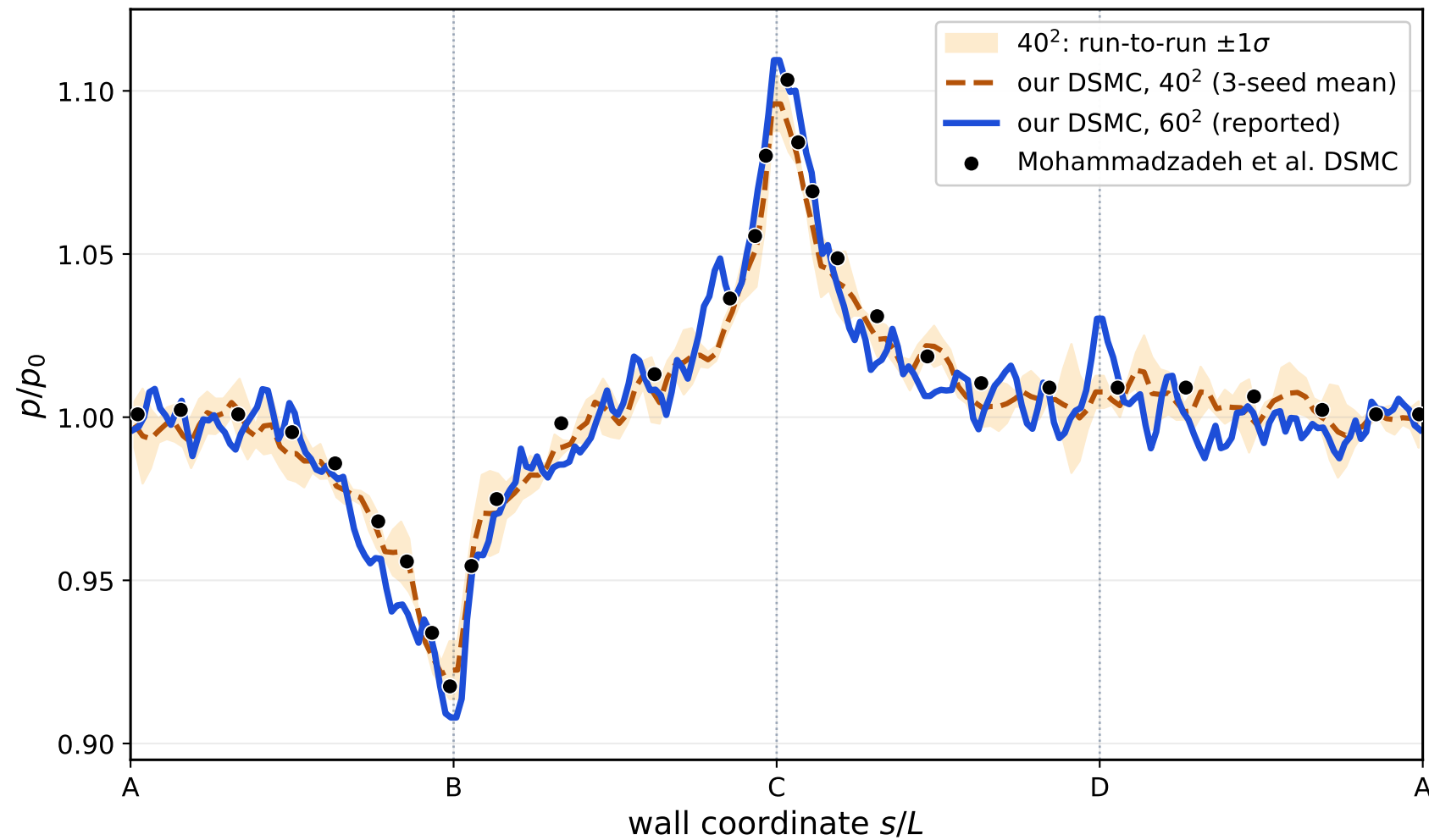
(a) Direct solver validation: Re = 1.5 , Kn = 0.1 , Ma = 0.09
