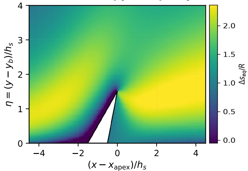
DSMC entropy-rise proxy
