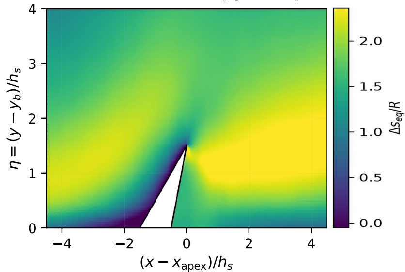
Reconstructed entropy-rise proxy
