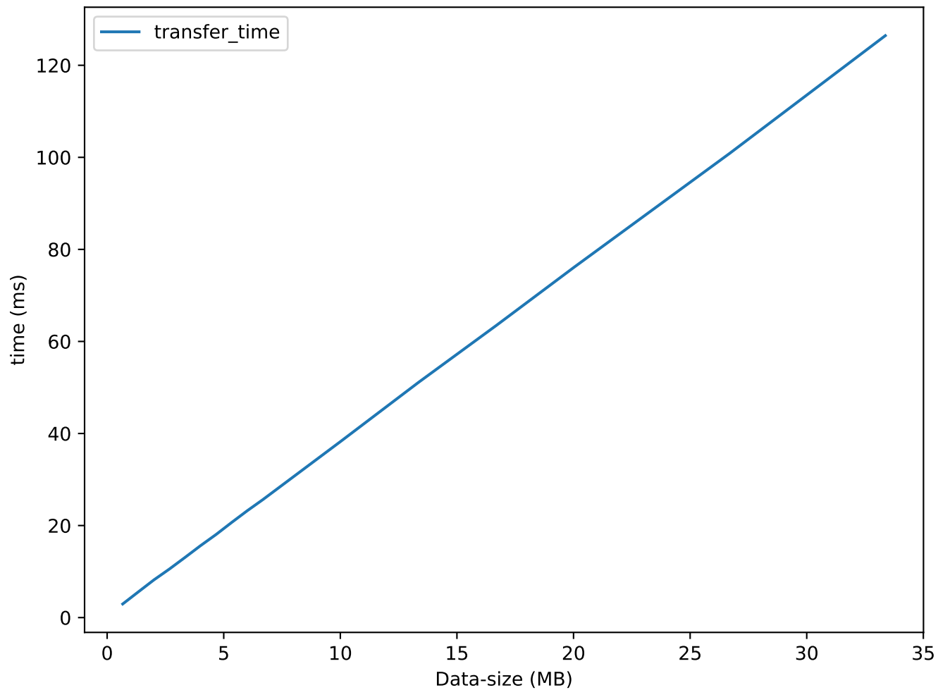
BL time vs Data size
