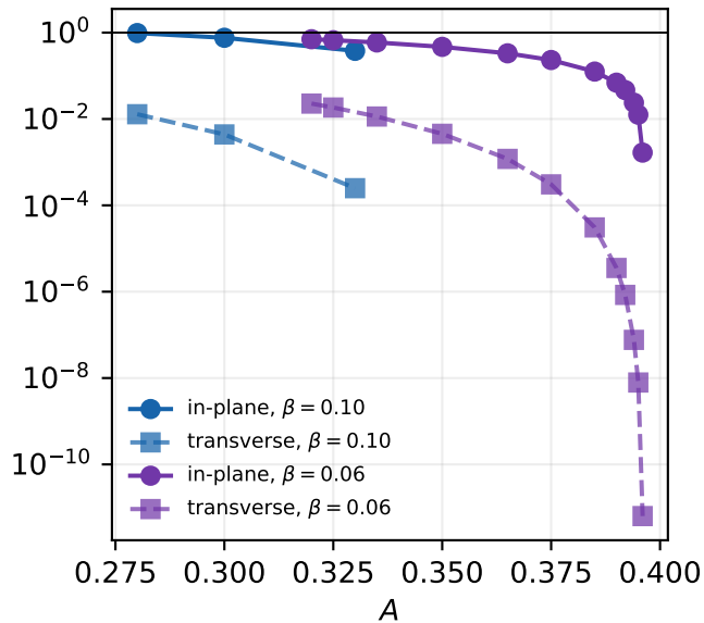
nontrivial Floquet multiplier
