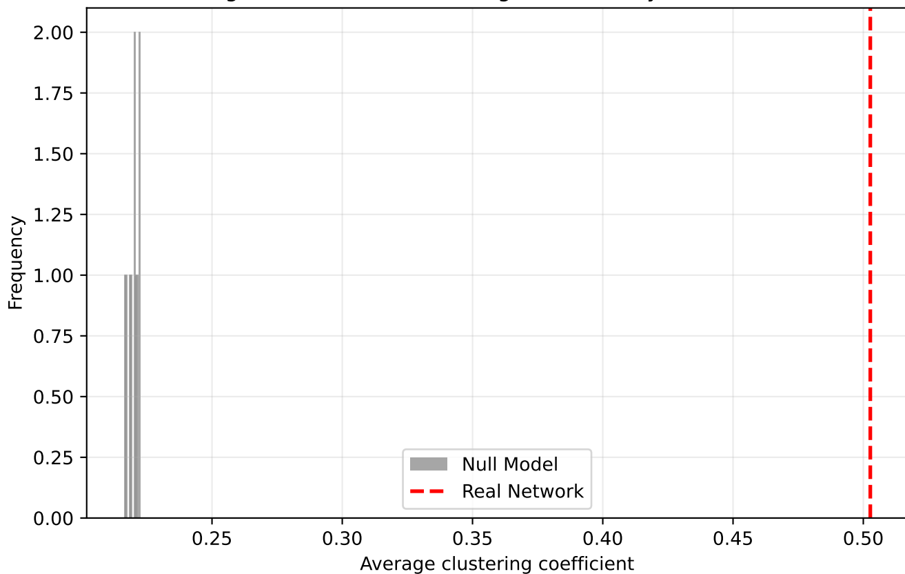
Configuration-Model Clustering (Citation-Layer) ( Z=142.86 )
