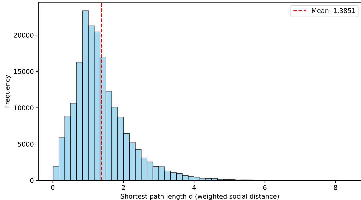
Cross-layer Path Distribution (Citation pairs in Social layer)
