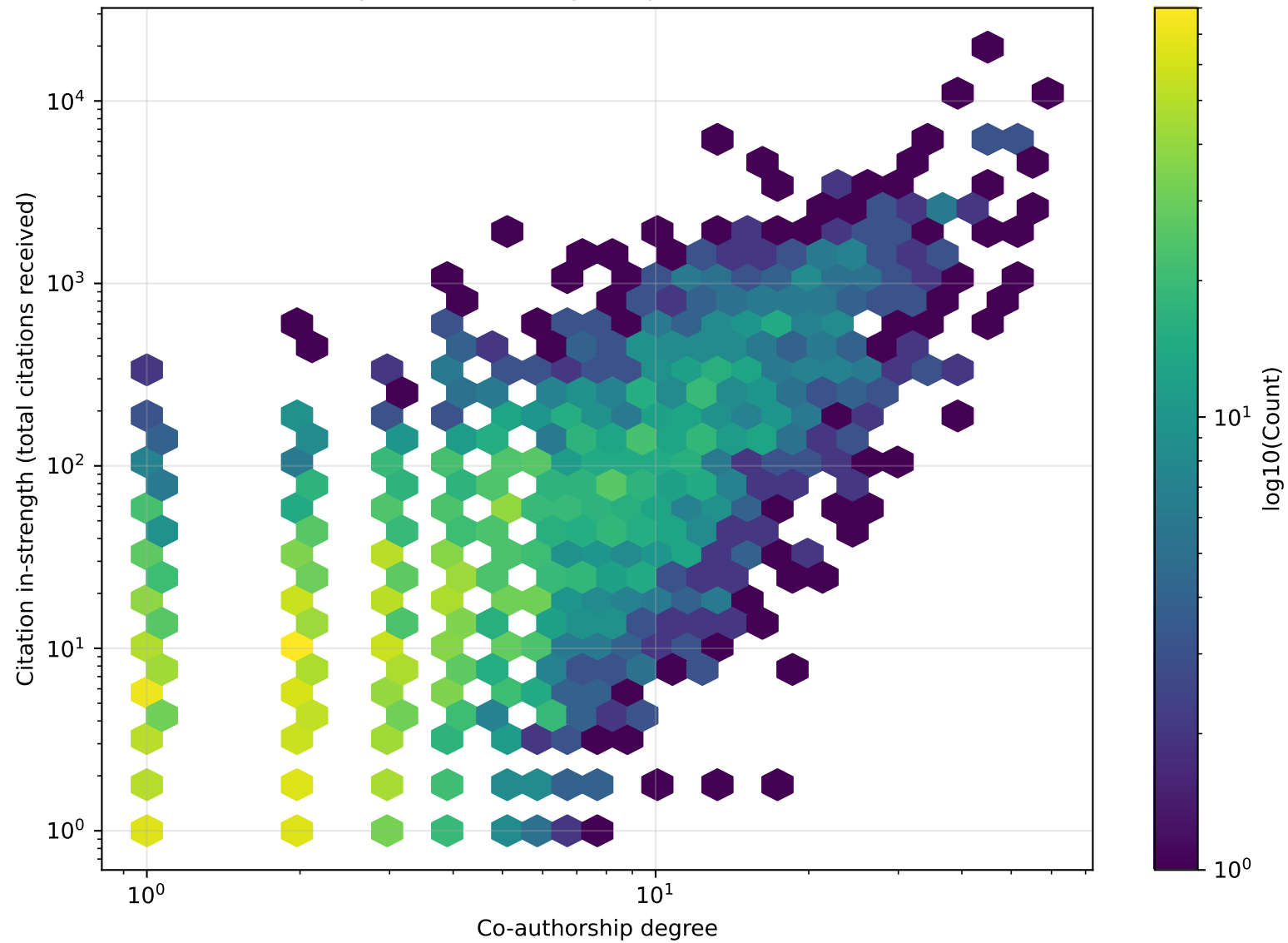
Degree vs In-Strength (Spearman r=0.65 )
