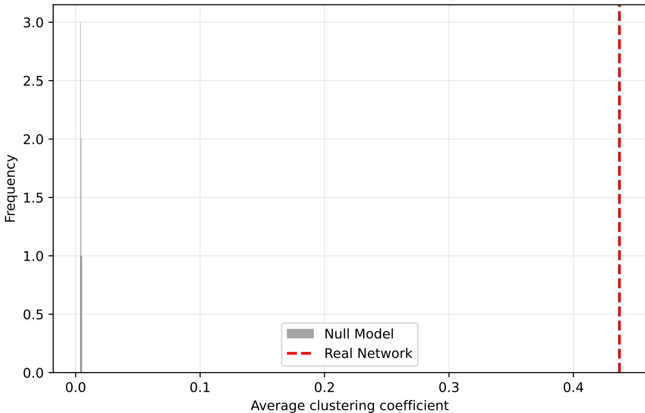
Configuration-Model Clustering (Social-Layer) ( Z=870.87 )
