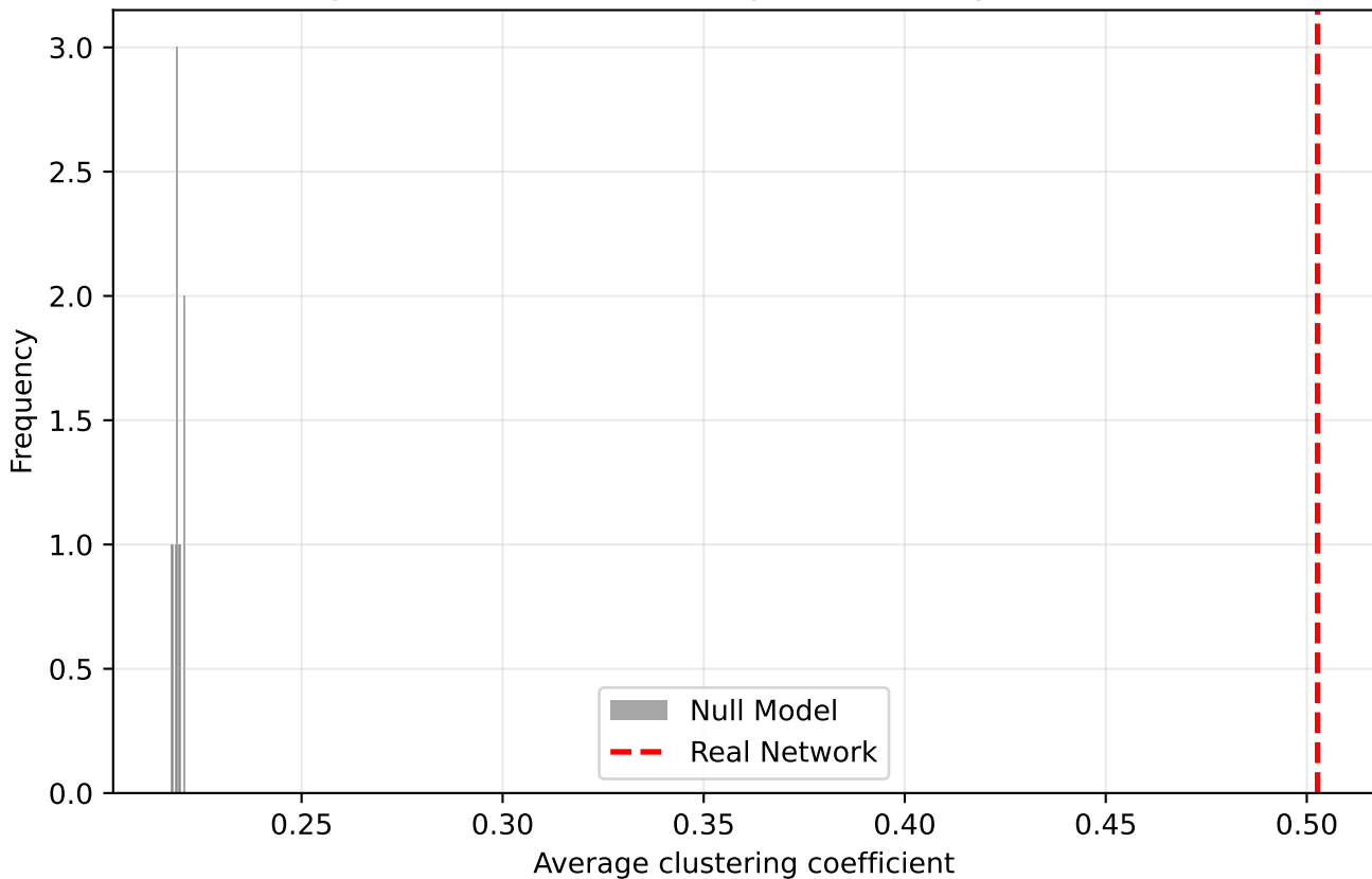
Configuration-Model Clustering (Citation-Layer) ( Z=259.69 )
