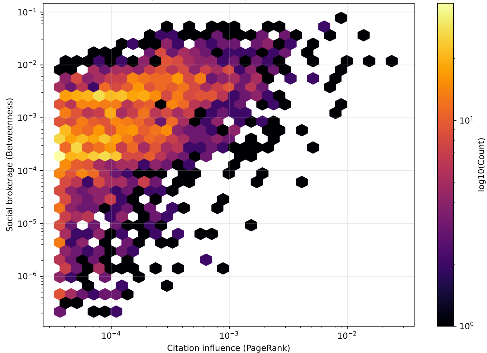
Multiplex Correlation (Spearman r=0.57 )
