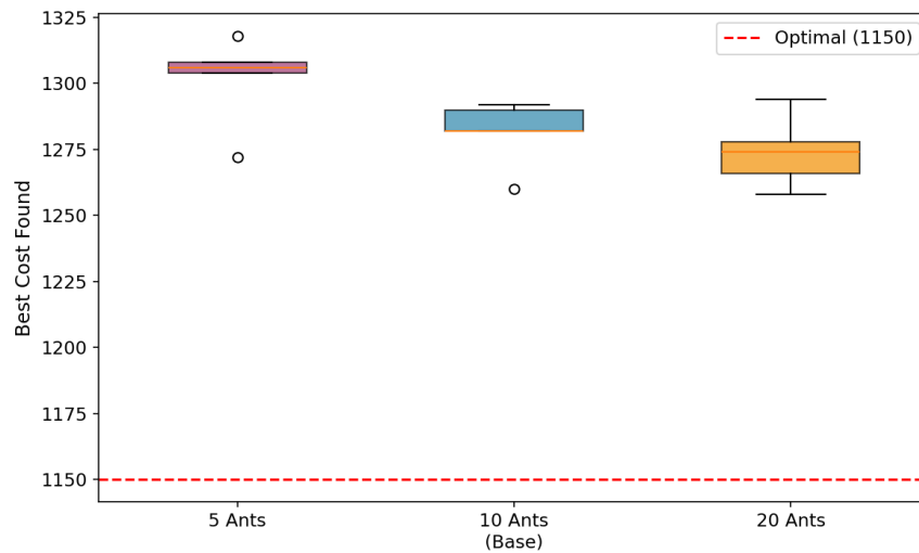
Figure 3: Boxplots of the population size experimentation
