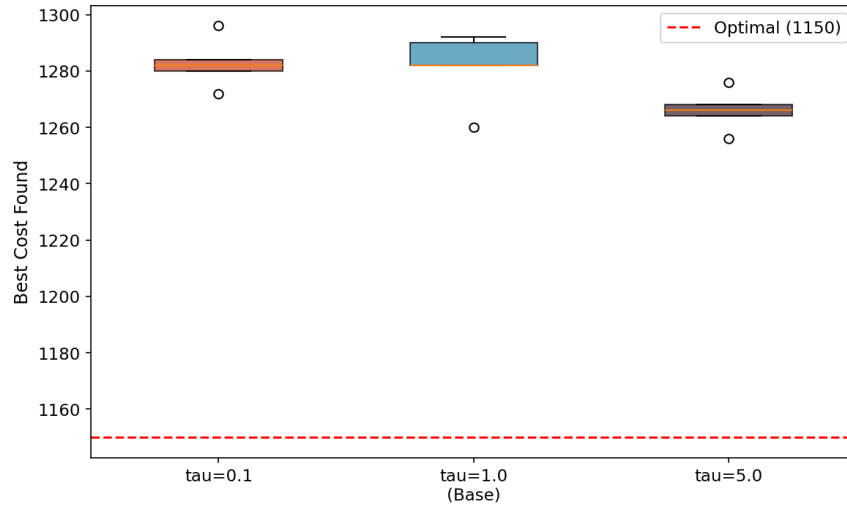
Figure 4: Boxplots for the initial pheromone experimentation
