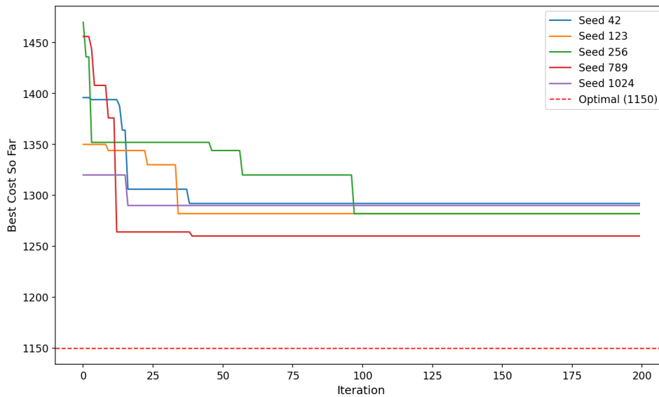
Figure 2: Convergence of best cost over iterations (Experiment 1)
