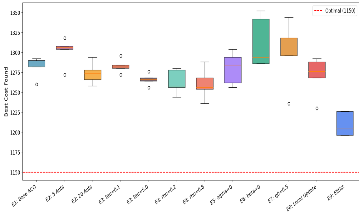
Figure 10: Best cost by ACO variant across all 60 runs
