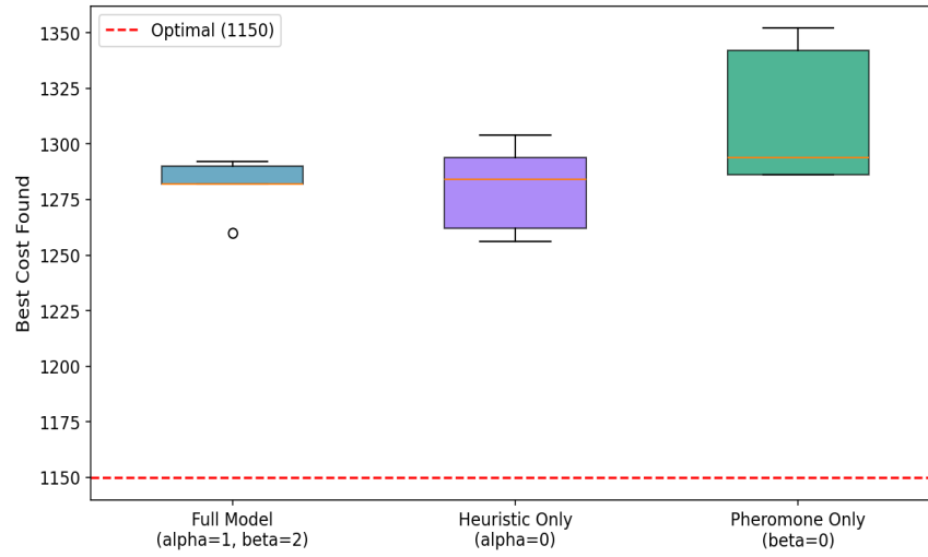
Figure 6: Boxplots for alpha and beta experimentation
