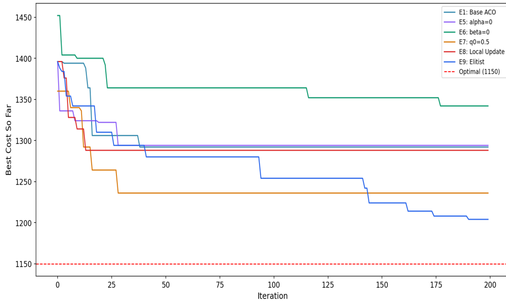
Figure 12: Convergence comparison across key ACO variants (Seed=42)
