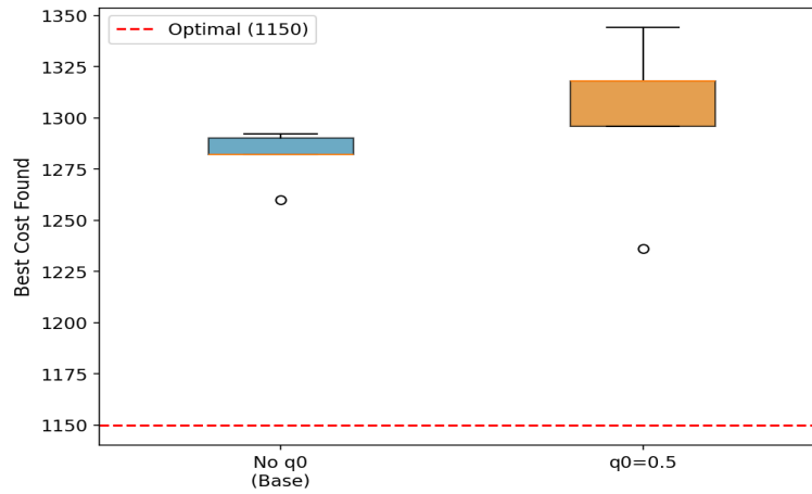
Figure 8: Boxplots with and without q_0 exploitation
