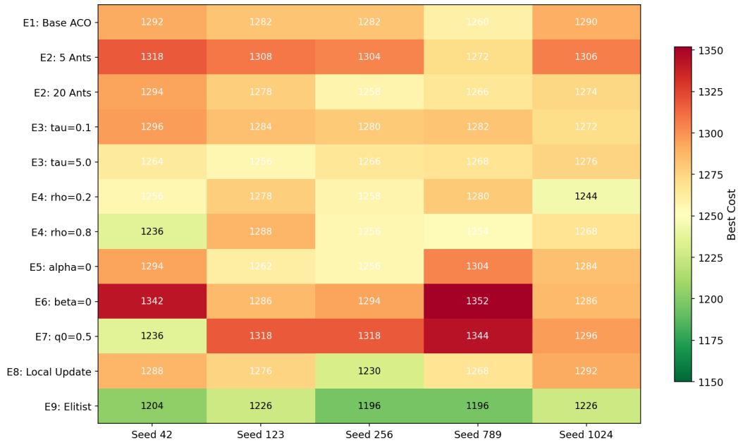
Figure 13: Best cost heatmap (Experiment vs. Seed)
