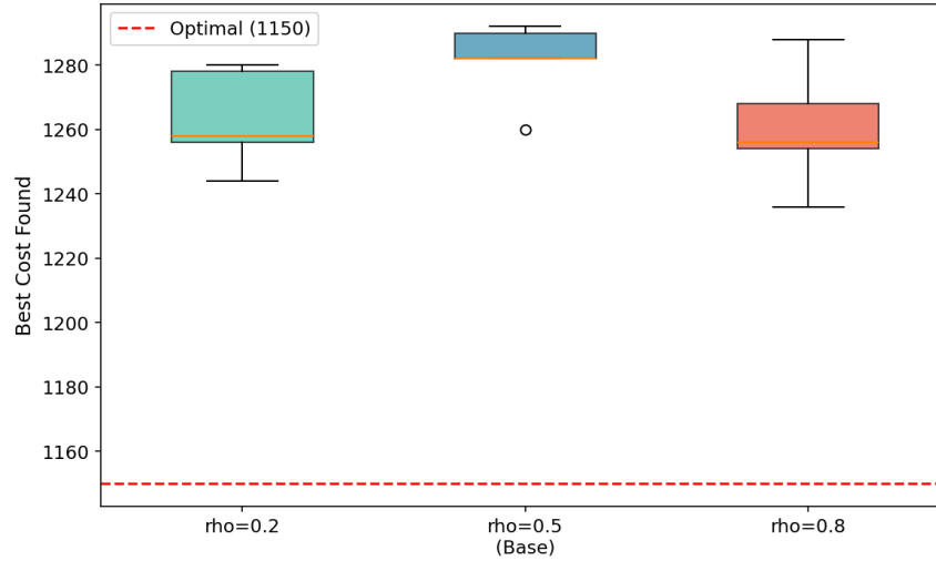
Figure 5: Boxplots for the evaporation rate experimentation
