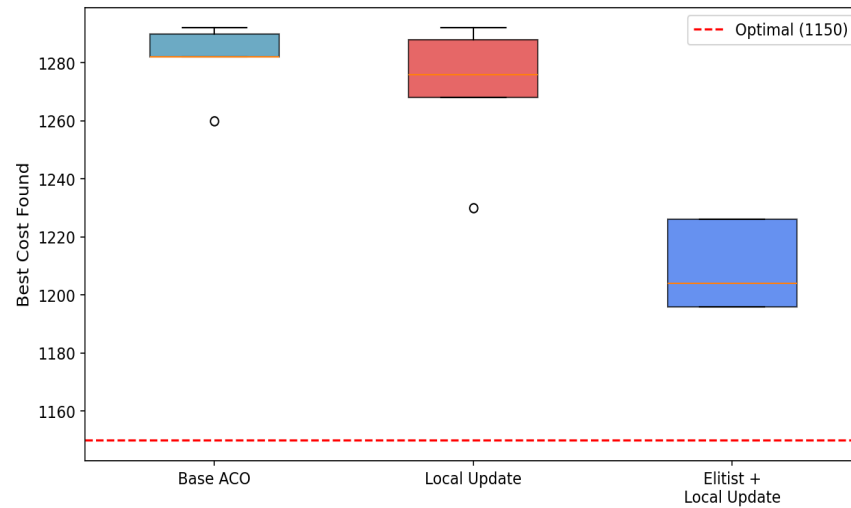
Figure 9: Boxplots comparing base, local update, and elitist strategies
