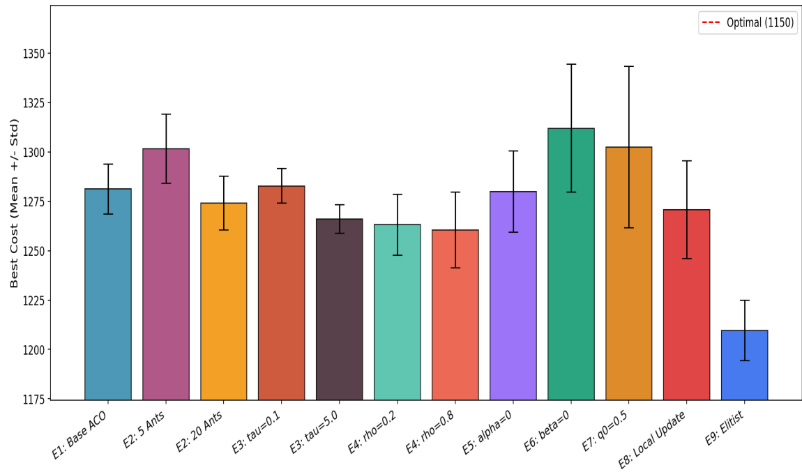
Figure 11: Mean best cost with standard deviation by experiment
