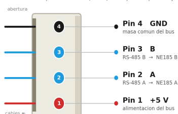
Conector 11 · MX 1.25 4P — RS-485 al NE185
