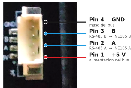
Conector 11 · MX 1.25 4P — RS-485 al NE185
