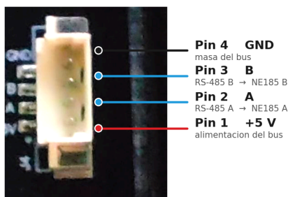
Conector 11 · MX 1.25 4P — RS-485 al NE185
