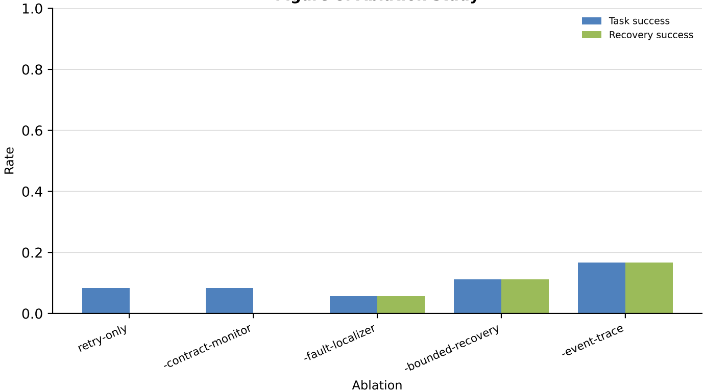
Figure 8: Ablation study
