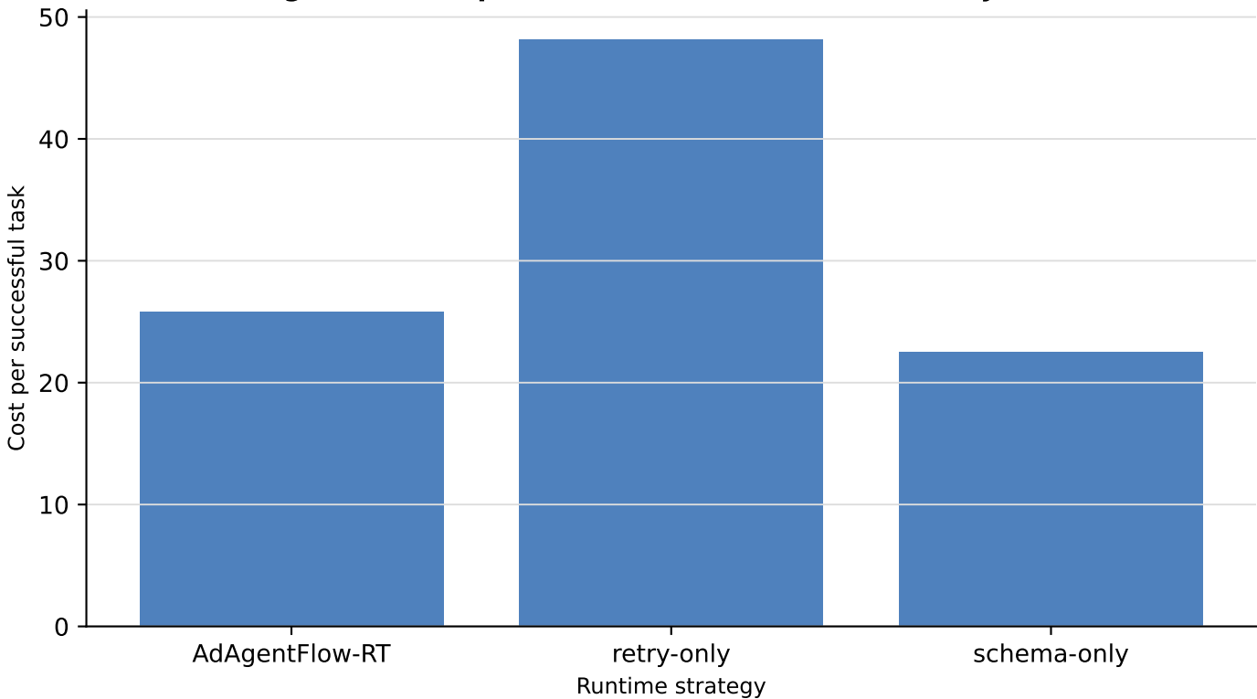
Figure 6: Cost per successful task under fault injection
