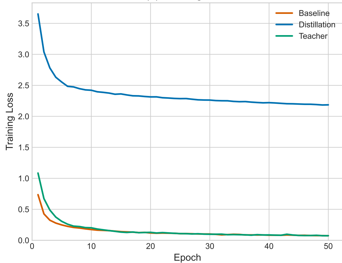
(a) Training Loss
