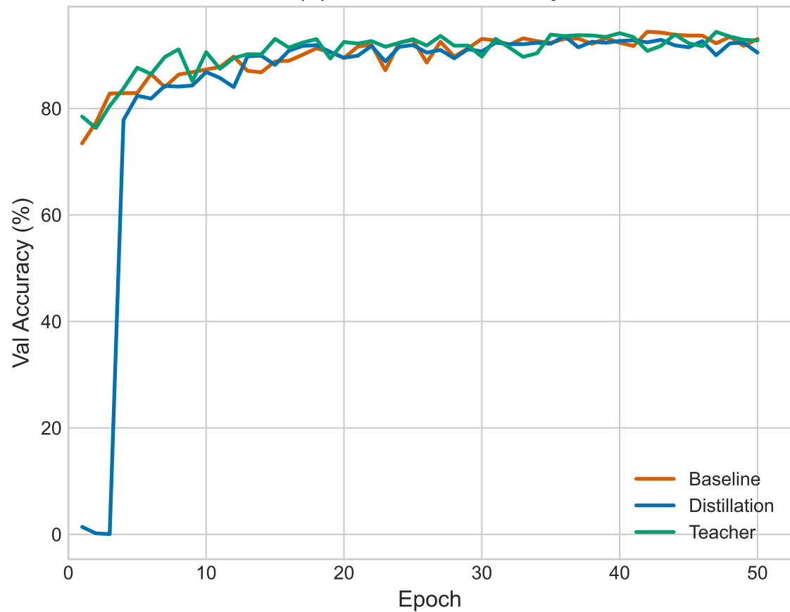
(b) Validation Accuracy
