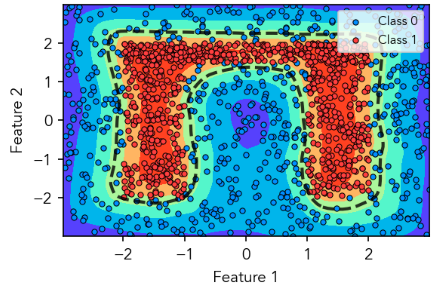
Base Learner: MLP (Iteration 4)
