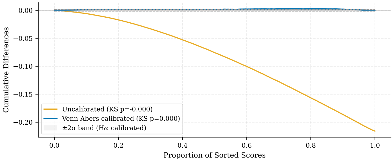
Calibration Hypothesis Test: Cumulative Differences (OOT, n = 276,869 )
