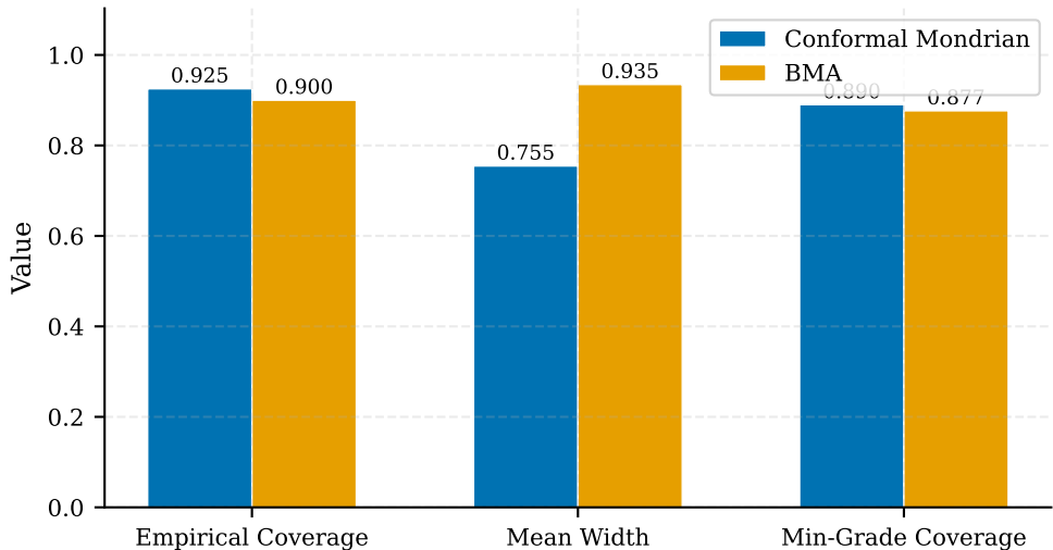
BMA vs. Conformal Mondrian: Uncertainty Interval Comparison
