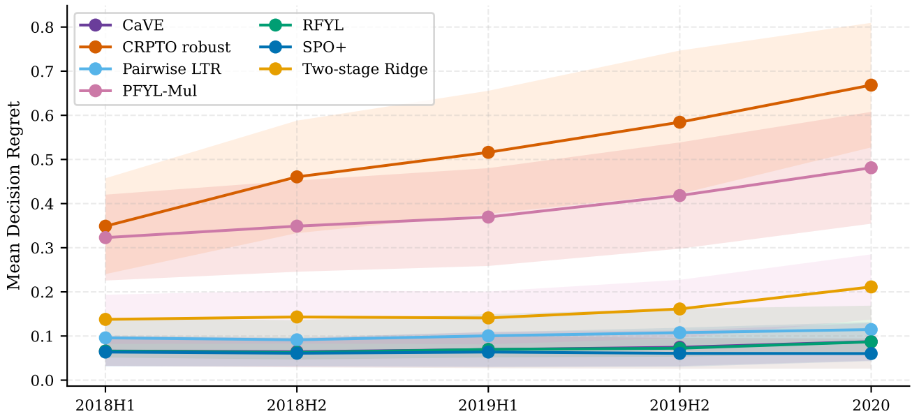
PyEPO Real Suite: Temporal OOT Stability
