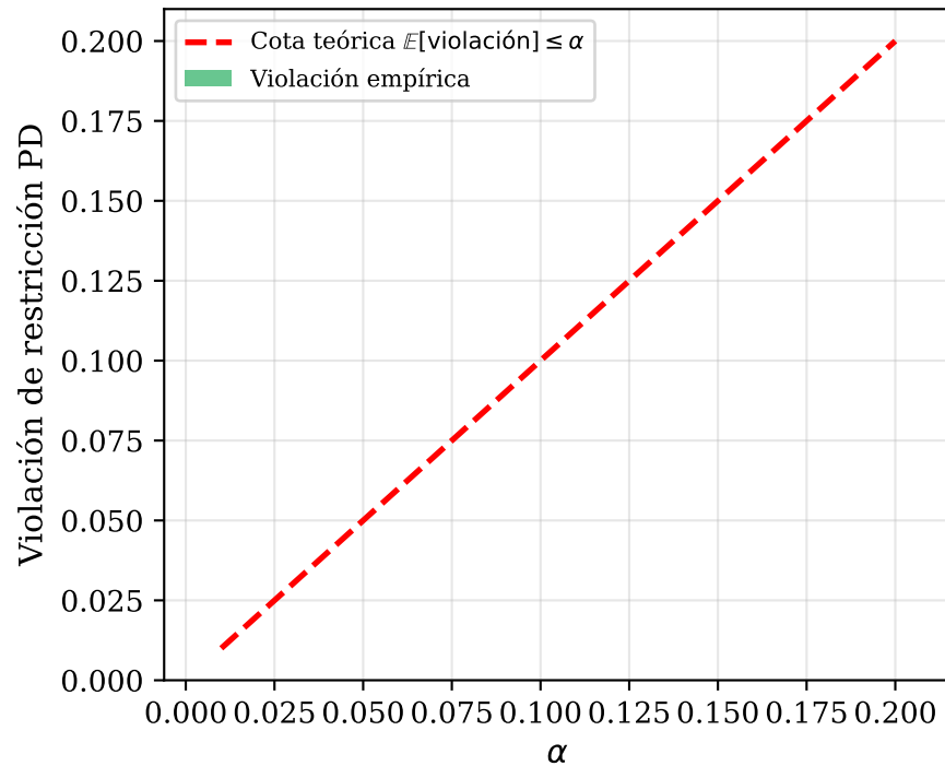
(B) Teorema 1(a): \mathbb{E}[\text{viol.}] \leq \alpha
