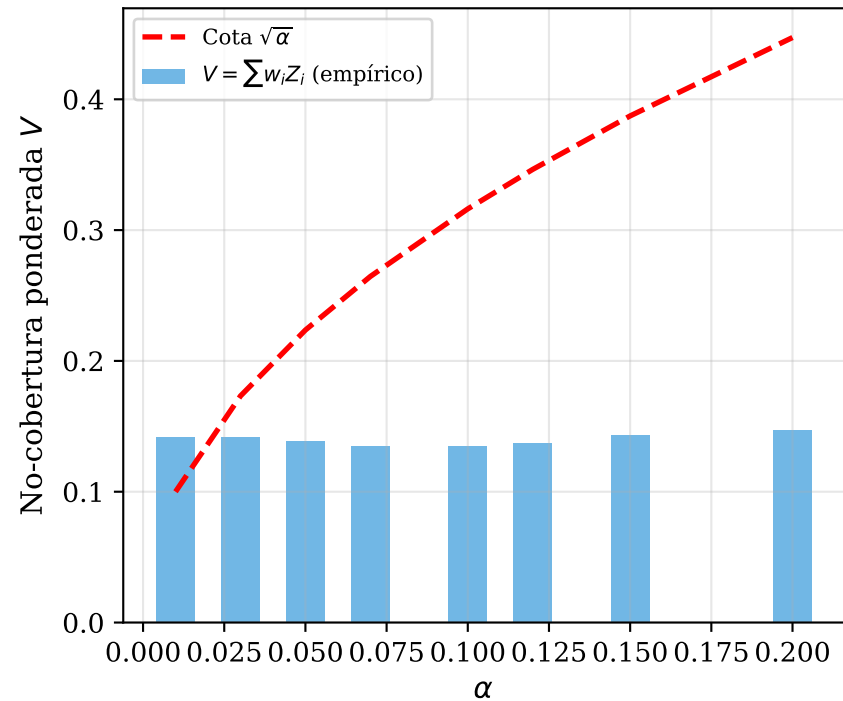
(C) Teorema 1(c): V \leq \sqrt{\alpha}
