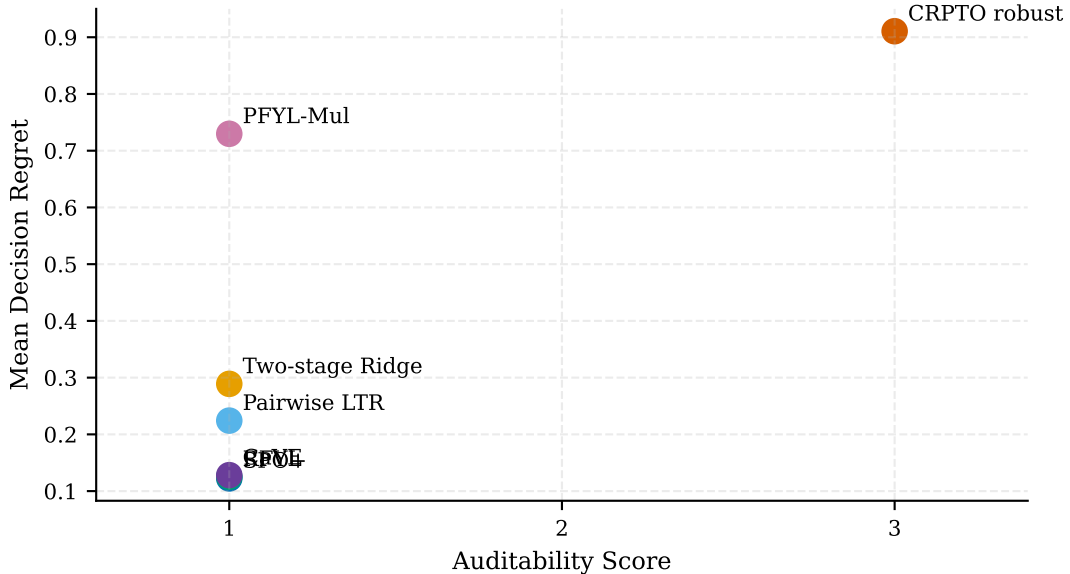
Regret-Auditability Frontier
