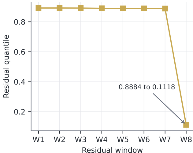
Applied conformal quantile
