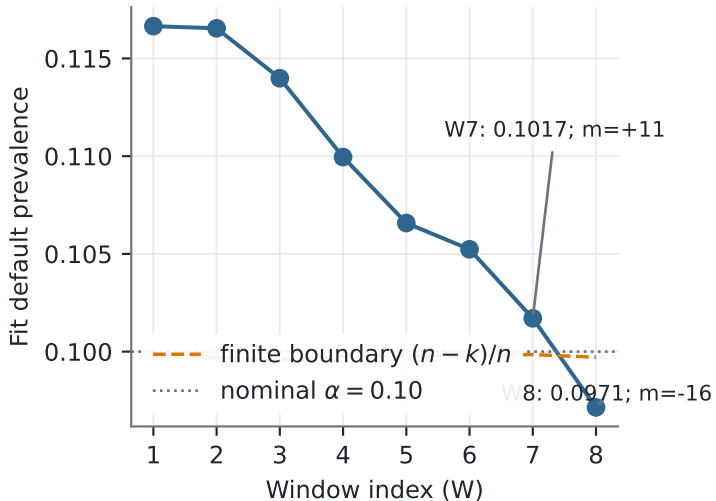
CatBoost S3 prevalence and phase boundary
