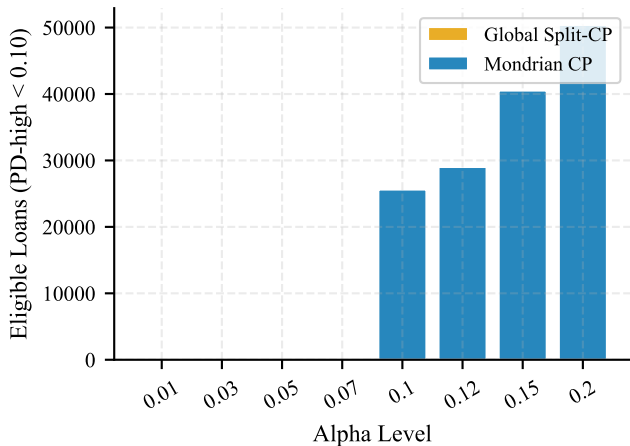
Eligible Loans vs. Alpha
