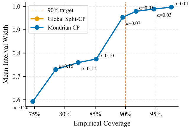
Coverage–Width Pareto Frontier
