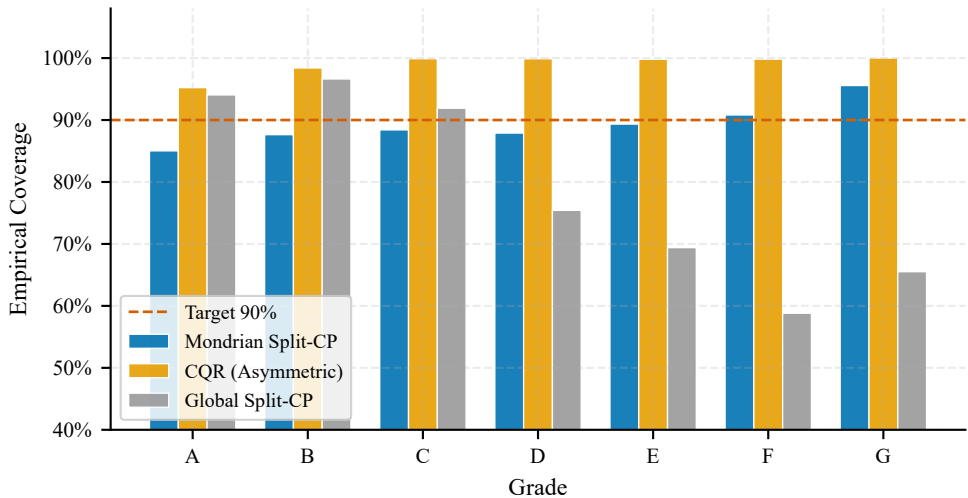
CQR vs. Mondrian CP: Per-Grade Coverage (OOT, \alpha = 0.10 )
