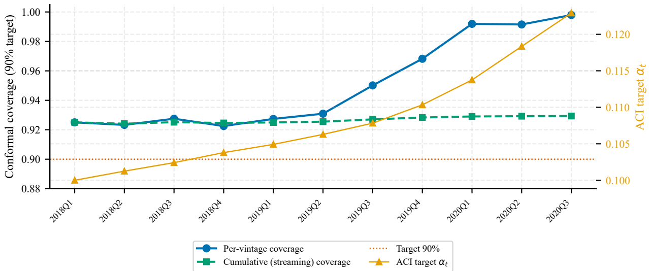
A24 — Online Conformal Stability Across the OOT Vintage Sequence
