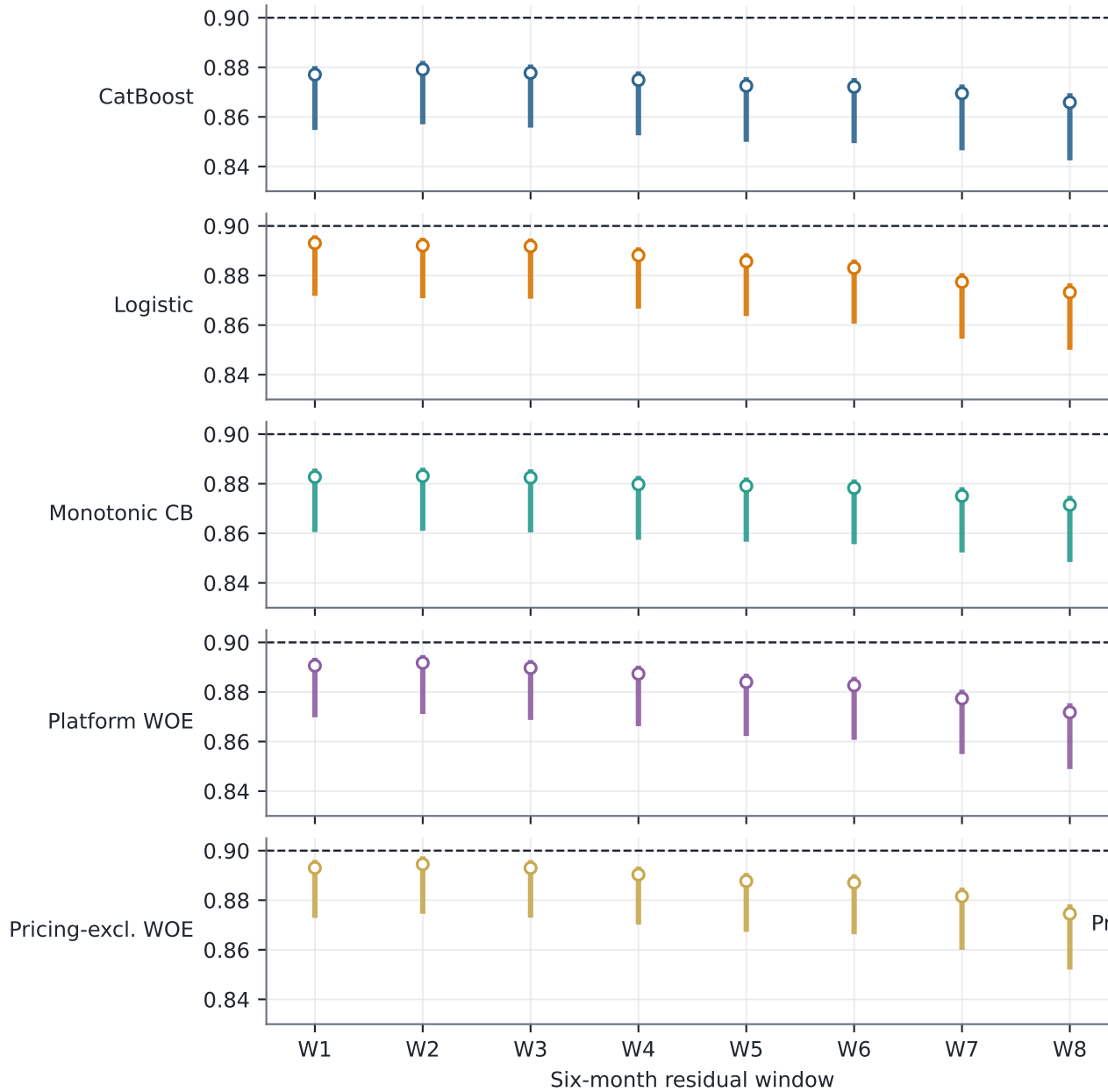
A. Resolved coverage (open dots) and sharp completion bounds (segments)
