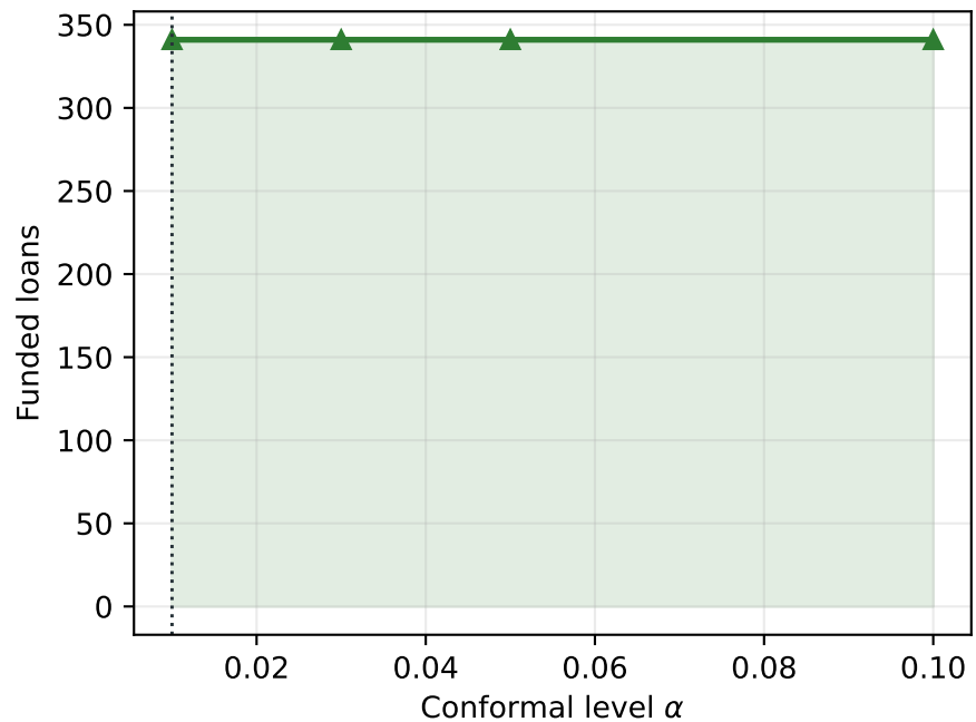
Funded-set size
