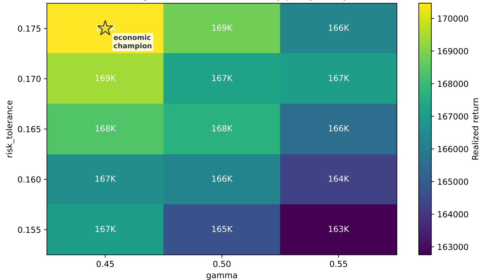
Robust region: best realized return by policy family
