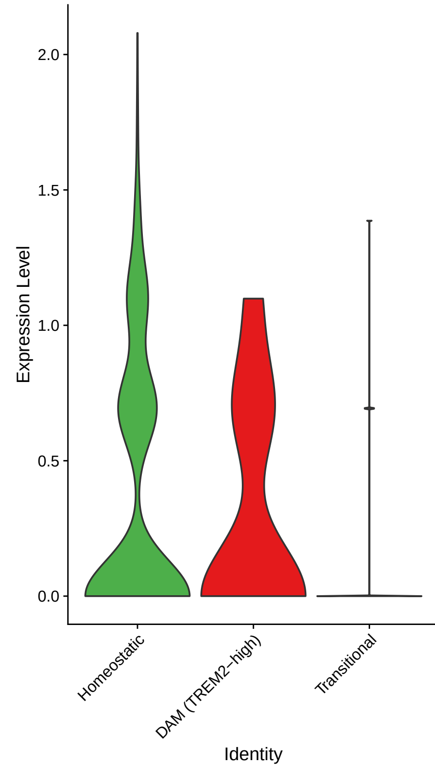
P2RY12
