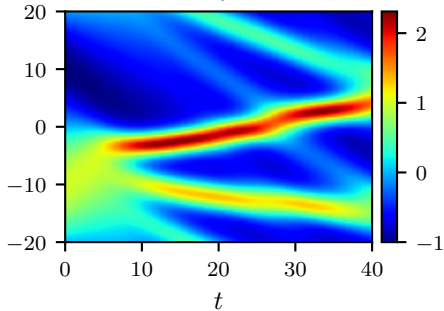
Exact Dynamics
