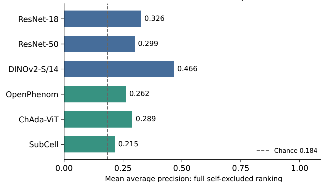
Yeast native markers · 10,499 crops · 9 classes
