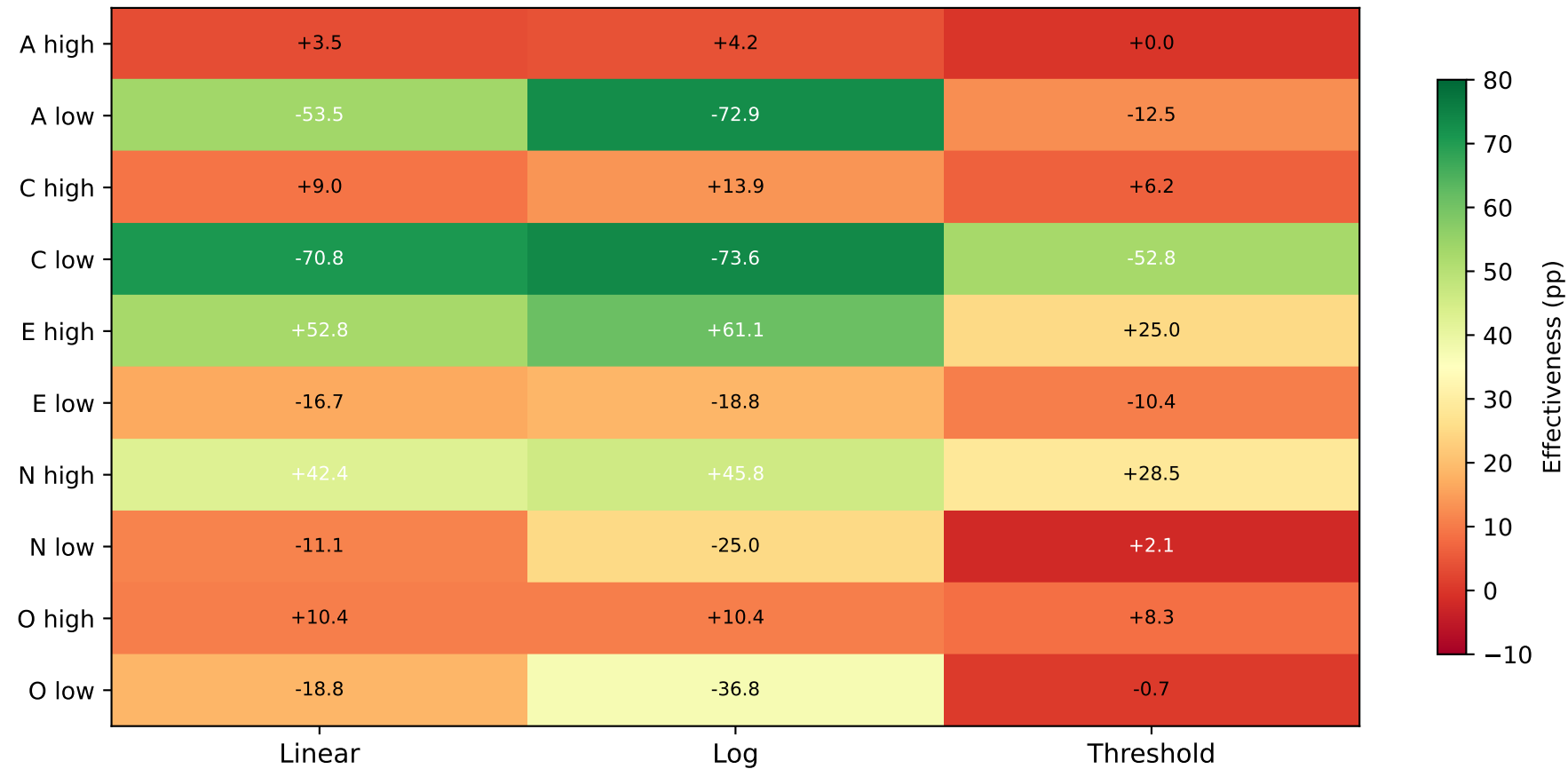
LATA Strategy Effectiveness (SCT): |\Delta_T| in Intended Direction (pp)
