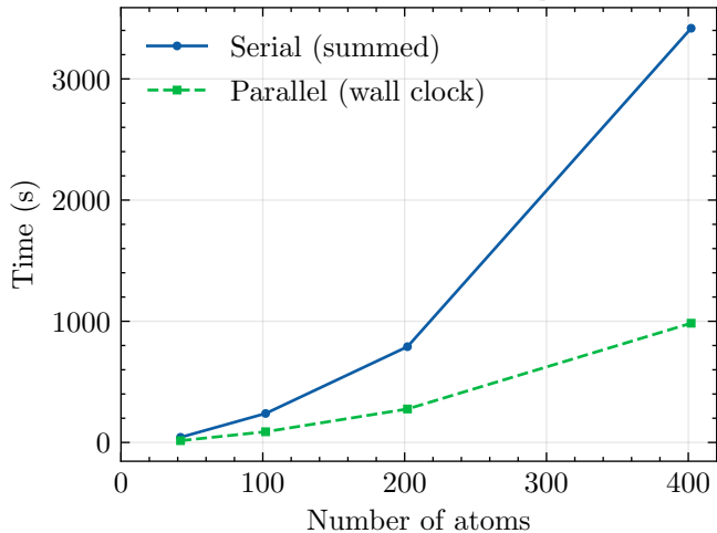
Wall time vs N_{atoms} ( n_{steps} = 10^6 )
