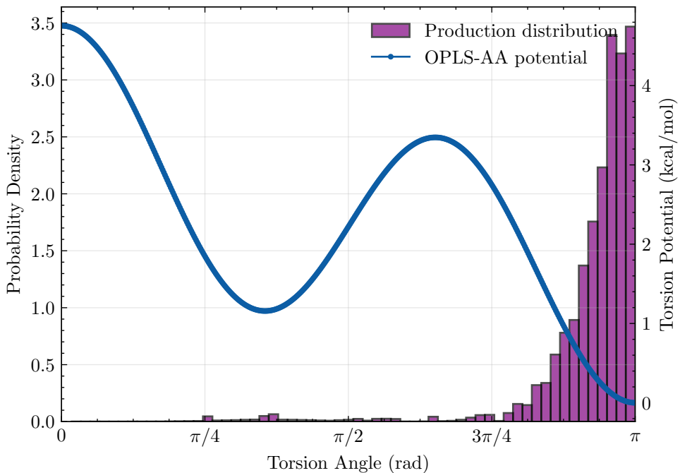
Production Torsion Distribution and Potential
