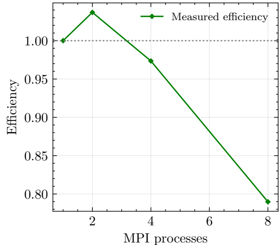
Efficiency vs np
