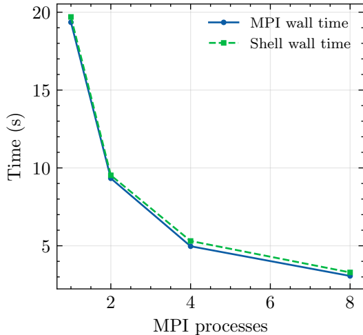
Wall time vs np
