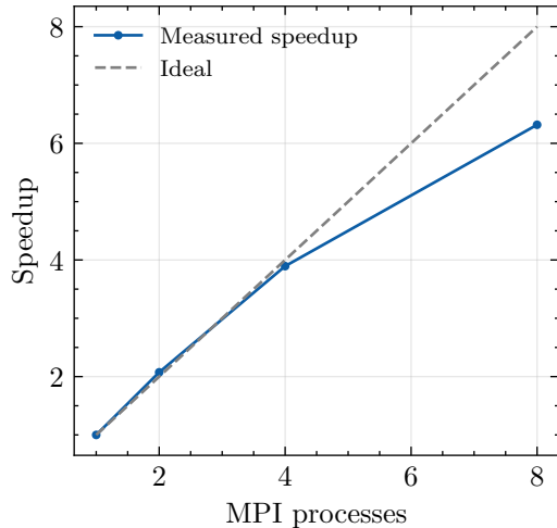
Speedup vs np
