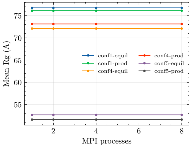
Rg vs np
