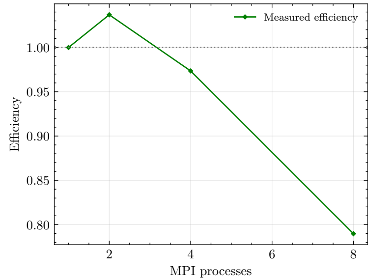
Efficiency vs np
