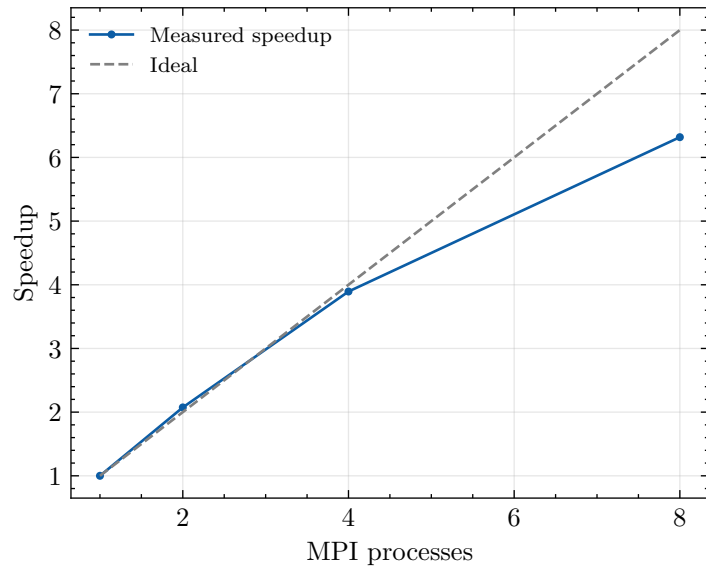
Speedup vs np
