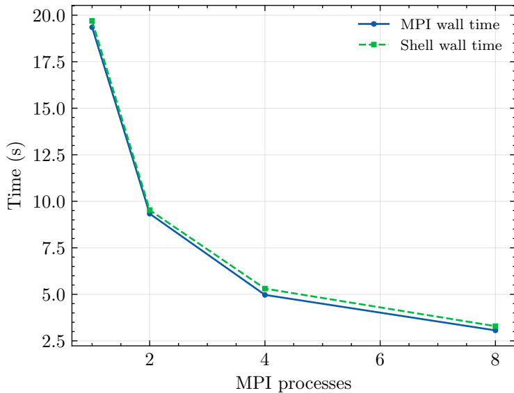
Wall time vs np
