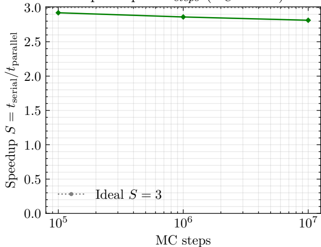
Speedup vs n_{steps} ( N_C = 100 )
